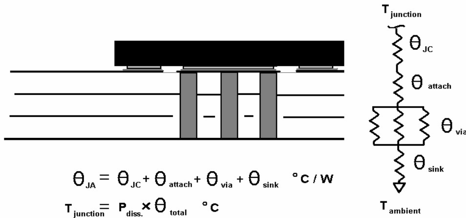
Figure 4 - PC board heatsink thermal model
