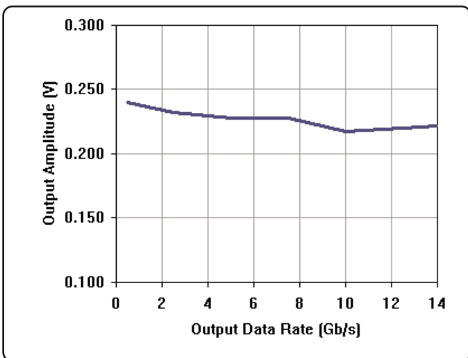
Figure 11: Data Output Amplitude vs Data Rate Power Supply @ -3.6V
