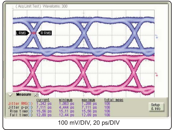
Figure 8: Data Output Eye Diagrams @ 14Gb/s Top: D3, Bottom: D4
