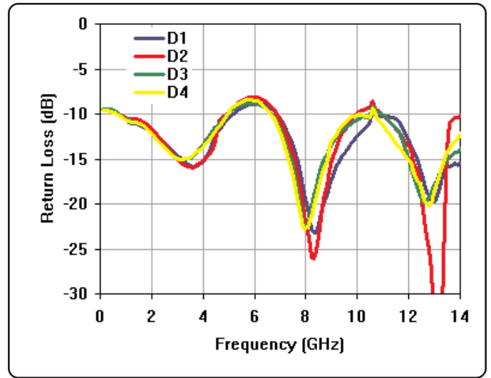
Figure 2: Data Output Return loss
