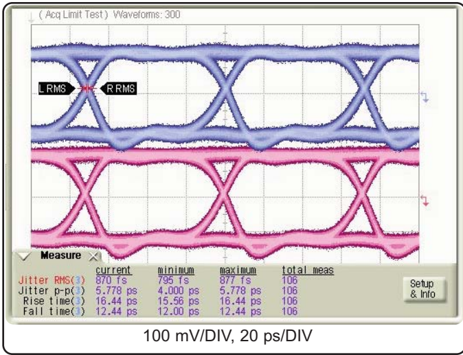
Figure 7: Data Output Eye Diagrams @ 14Gb/s Top: D1, Bottom: D2
