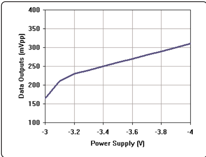
Figure 9: Data Output Amplitude vs Power Supply Output Data Rate @ 10Gb/s
