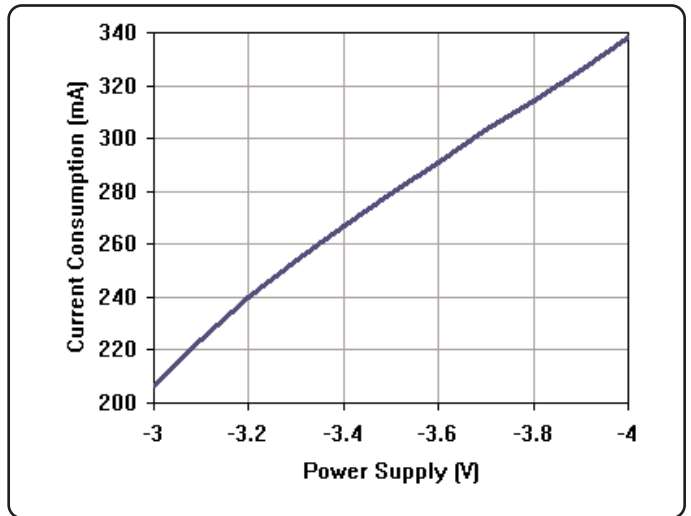
Figure 10: Total Current Consumption vs Power Supply Level
