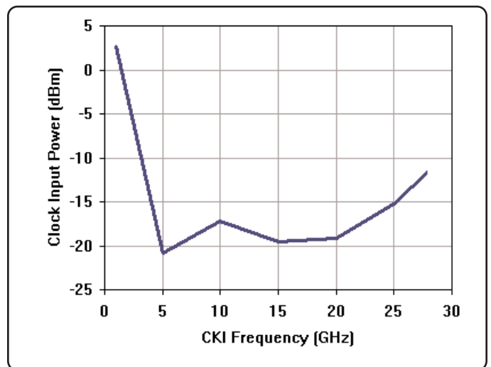
Figure 12: Clock Input Sensitivity vs Frequency Power Supply @ -3.6V
