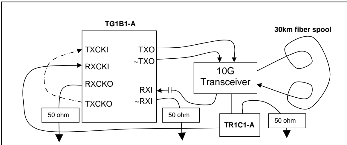
Fig. 1 Optical Single-Ended Loop Back Test with CRU
