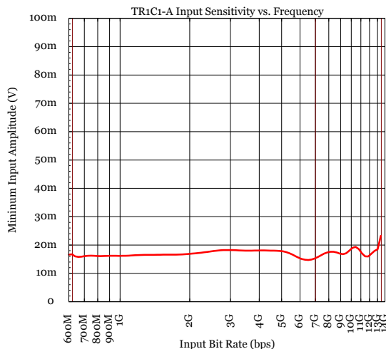
Figure 5 - Typical Input Sensitivity
